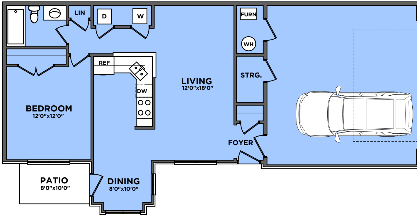
FLOOR PLAN A-1 1 BEDROOM 1 BATH 980 SF FIRST FLOOR
