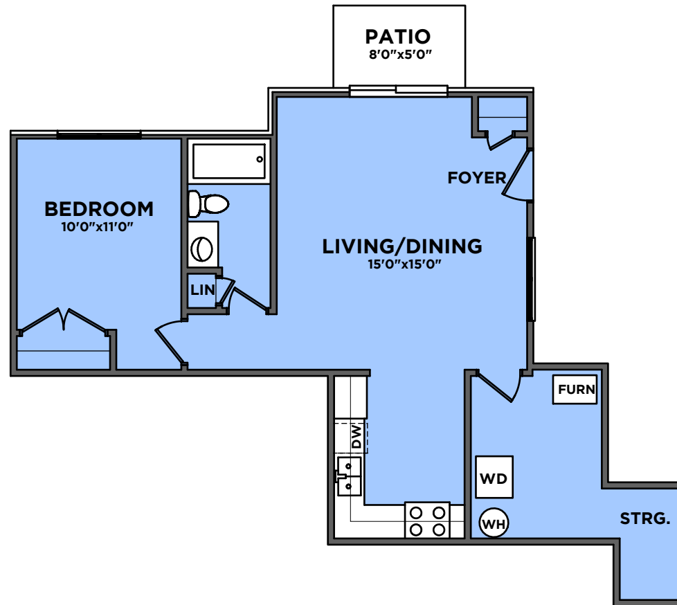
FLOOR PLAN BL 1 BEDROOM 1 BATH 880 SF
